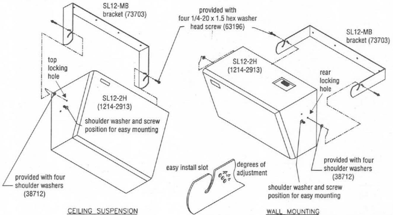
Figure 1—Mounting
